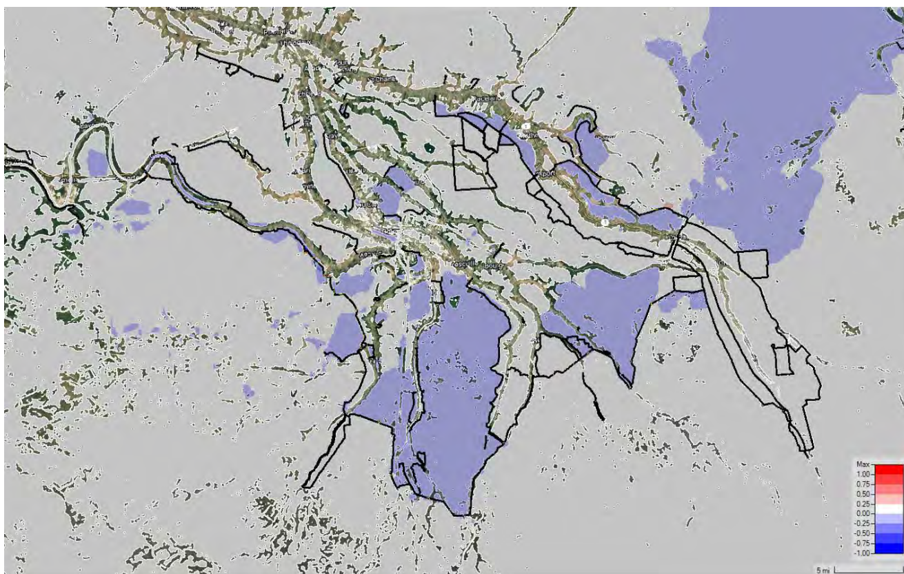
Figure H:1-1. 5-Year Event in the 2035 Condition Comparing FWP-FWOP
